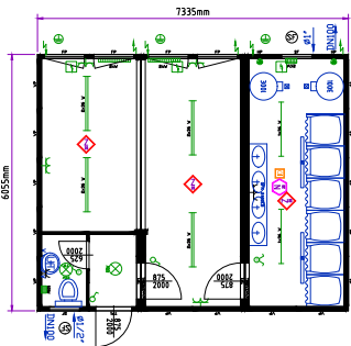
Office and sanitary cabin 3 units
