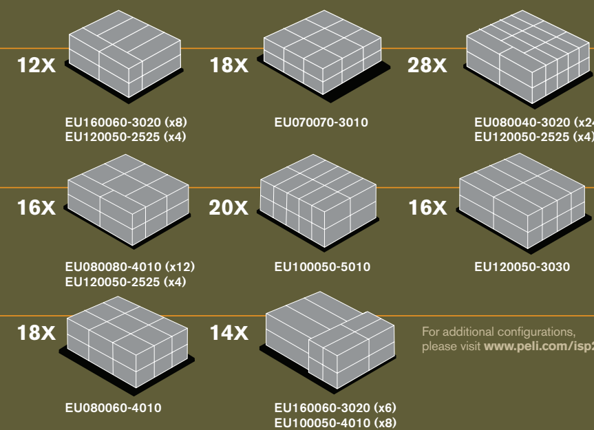
463L Master Pallet case configuration examples
