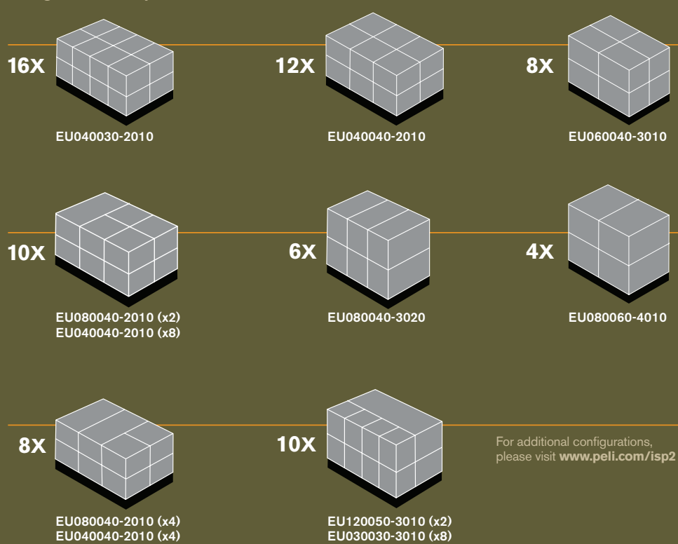
Euro Pallet case configuration examples
