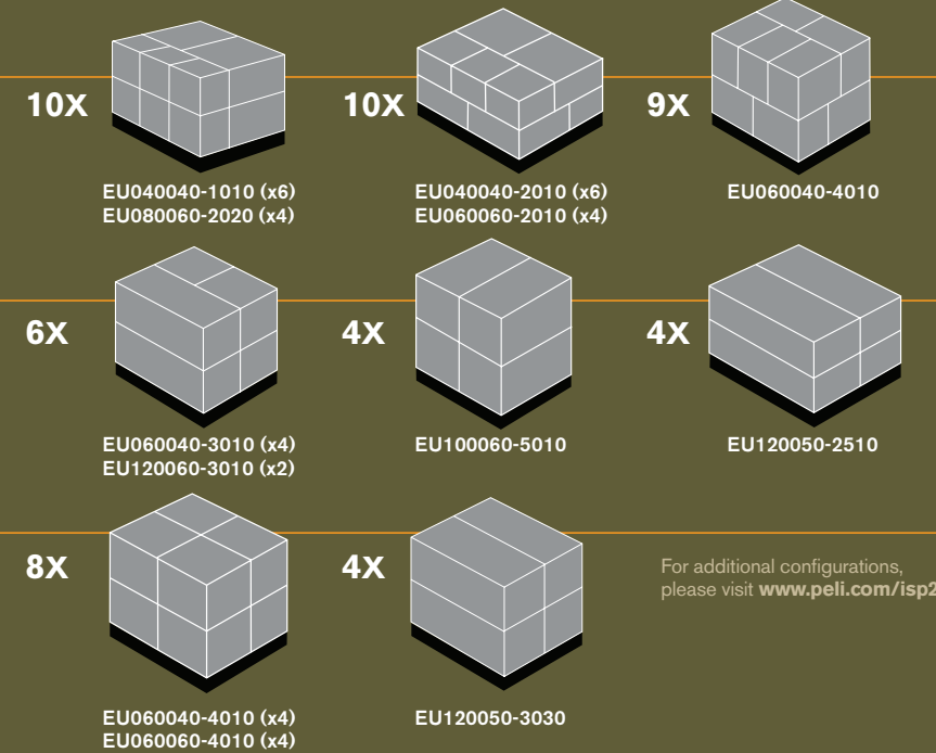
US Nato Pallet case configuration examples
