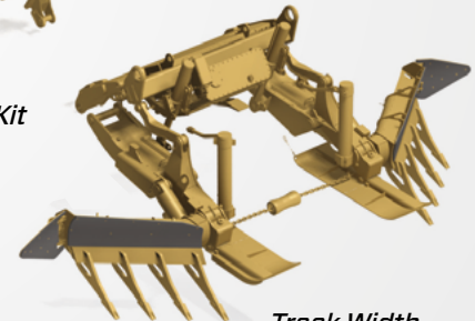
Track Width Mine Plough
