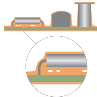
Liquid Coating
