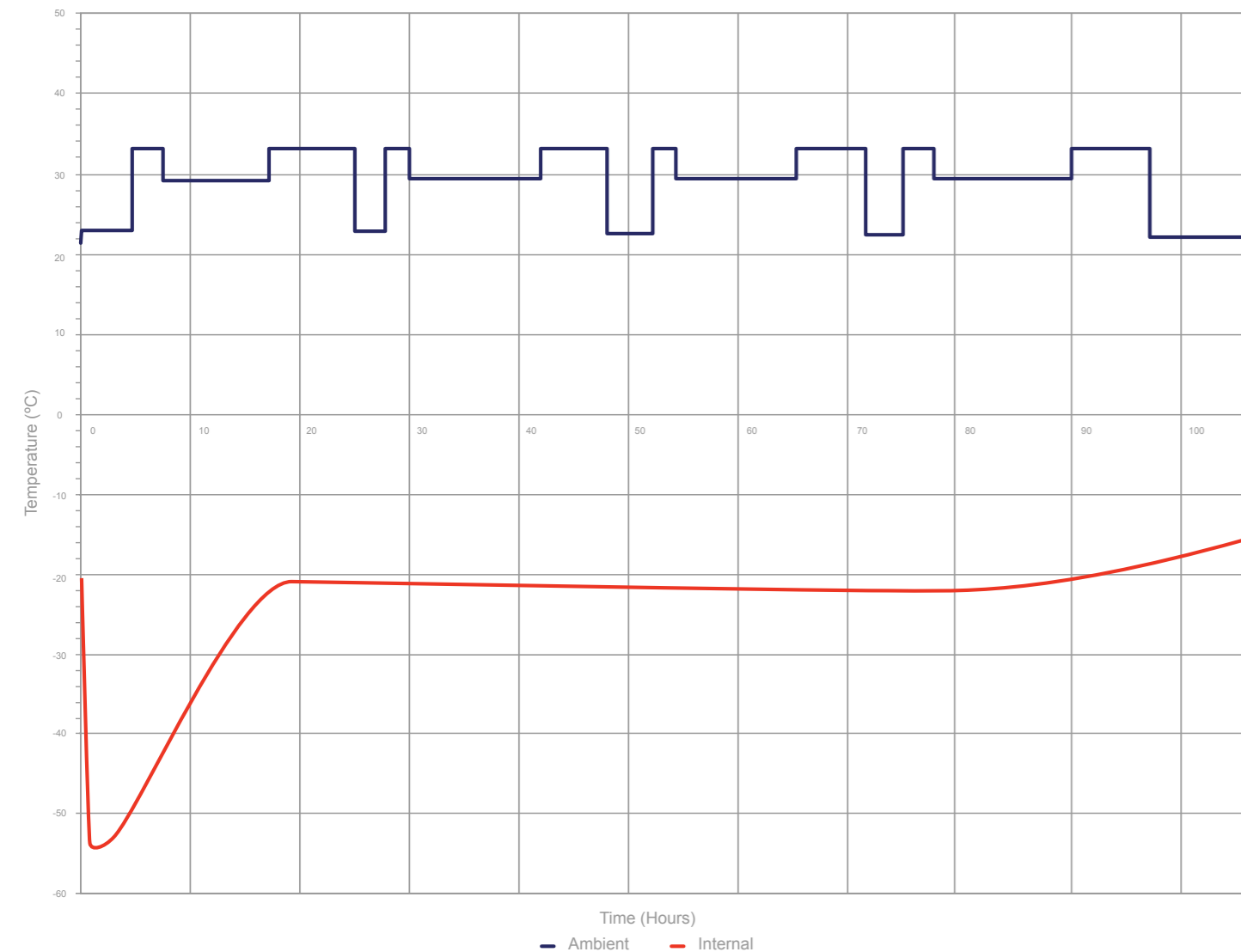
Series 20M 2896 ISTA Summer Thermal Performance
